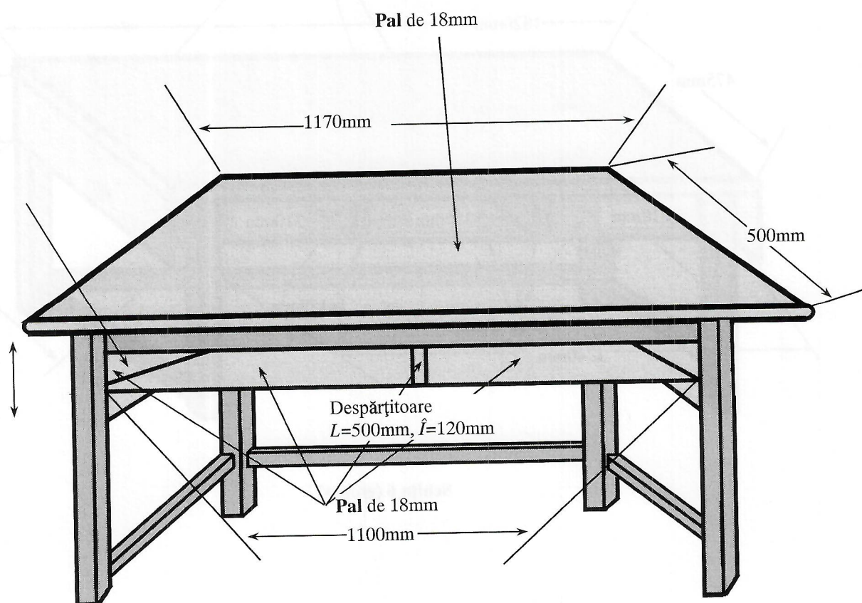
Schița 7 (propus)
