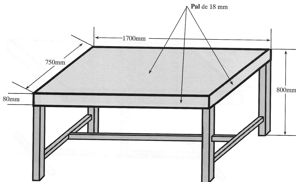
Schița 8 (propus)
