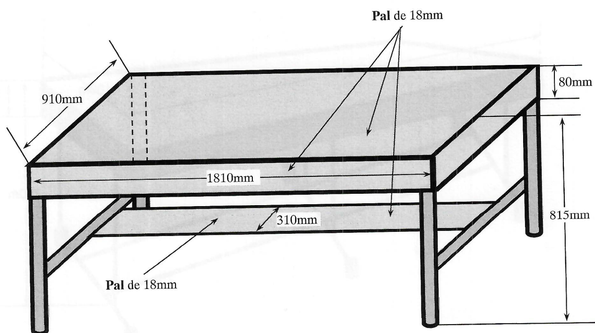
Schița 3 (propus)
