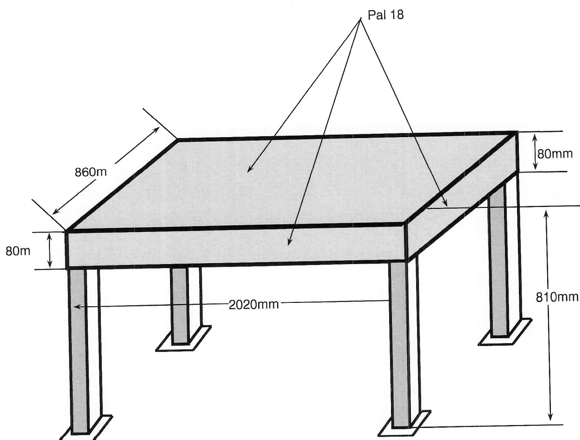
Schița 1 (propus)
